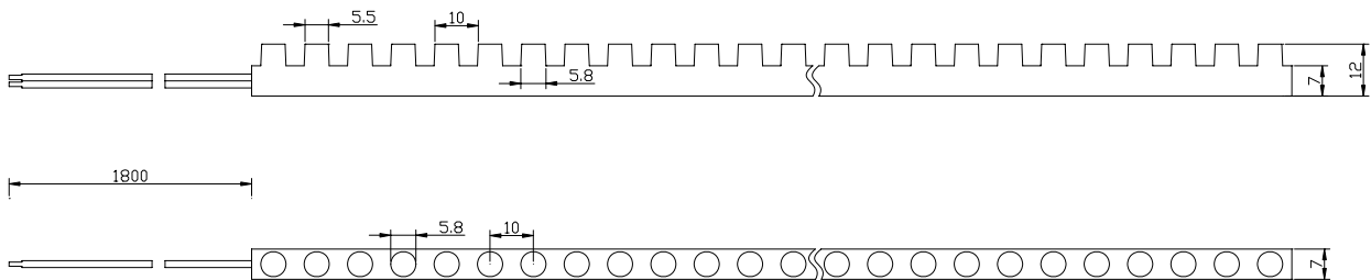
MODEL: RX-LED24 3mm Round without flange LED strip (clear PVC-waterproof)
