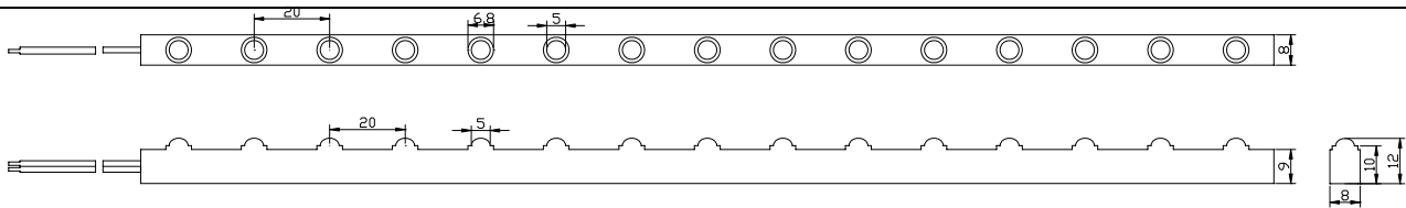
MODEL: RX-5MM15-5H 5mm Starw hat LED water clear PVC flexible strip LED light
