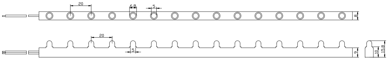
MODEL: RX-5MM15-5K 5mm Round LED water clear PVC flexible strip LED light
