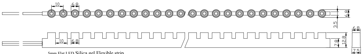
5mm Flat LED Silica gel Flexible strip MODEL:RX-LED96(RX-SI10-96-5MM)
